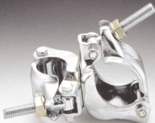
φ60.5×φ48.6
